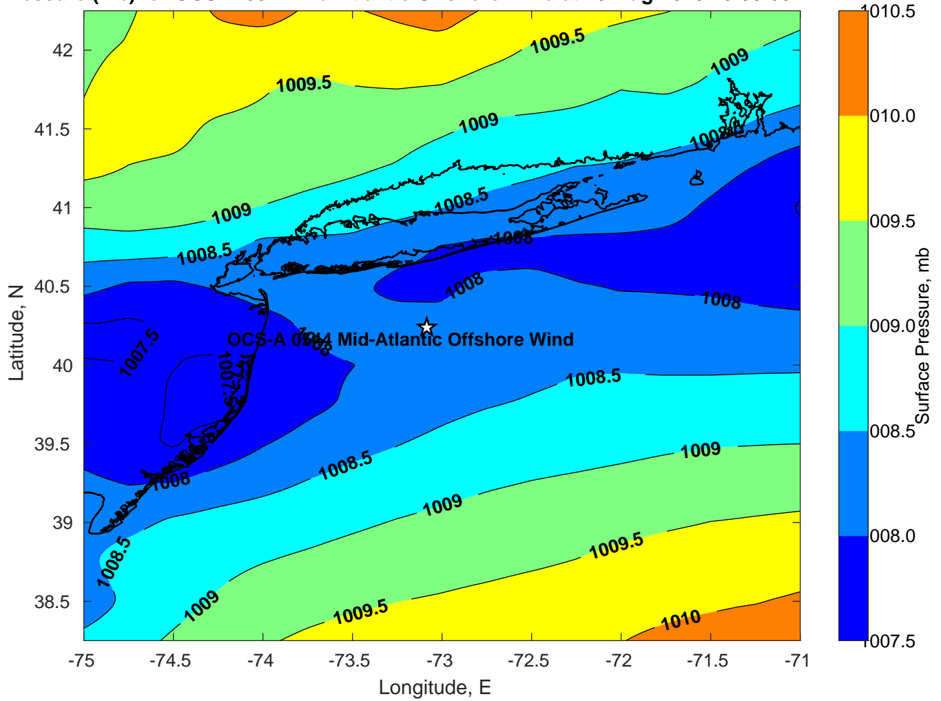
Surface Pressure (mb) for OCS-A 0544 Mid-Atlantic Offshore Wind at 15-Aug-2023 18:00:00
